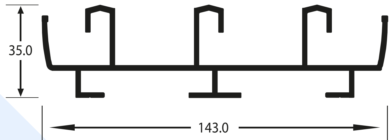
Marco triple corrediza
