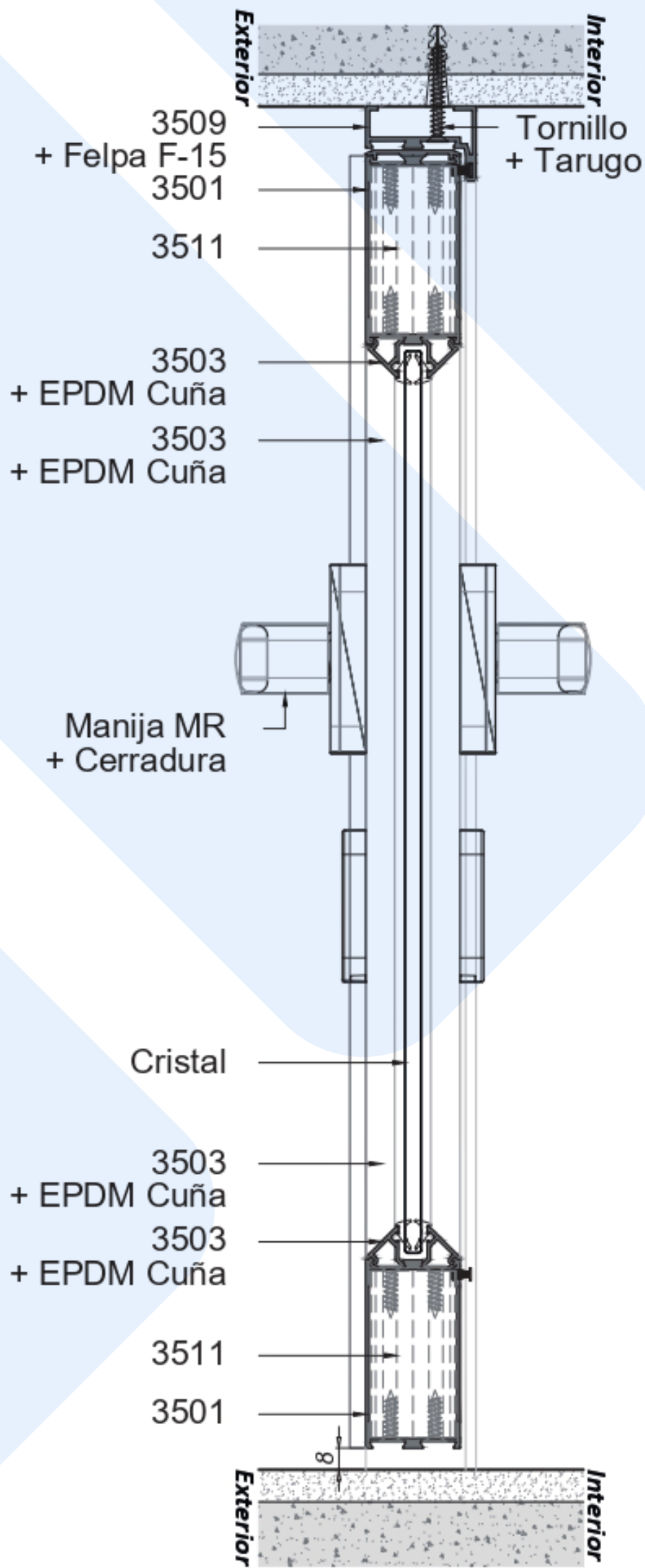
Vista vertical
