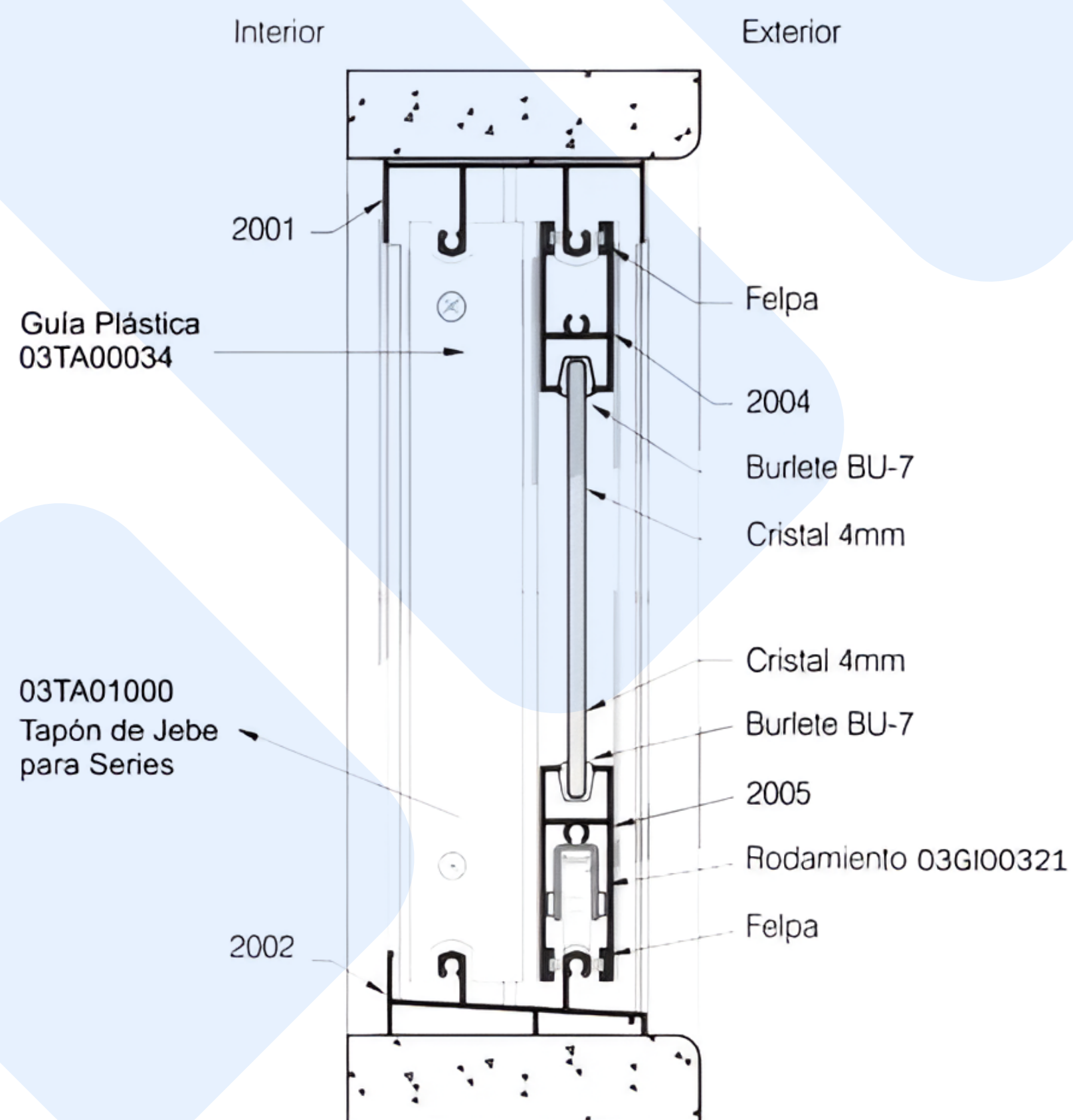
Vista vertical
